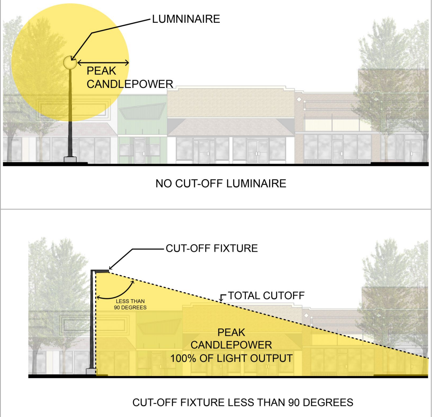
Figure 1204.31-1, Free-Standing Luminaires Examples
